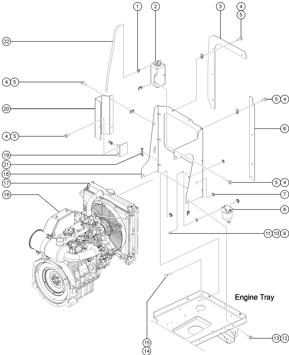
402.1 Kubota D1105-E4B, View 1
